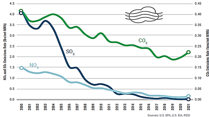
Emission Rates from Electric Generation in New York: 2000-2021
